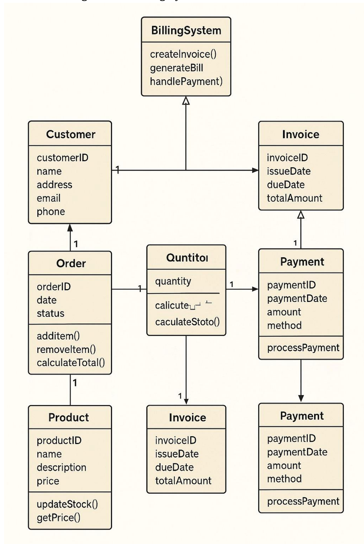
5.8 UML Class Diagram for Billing System
