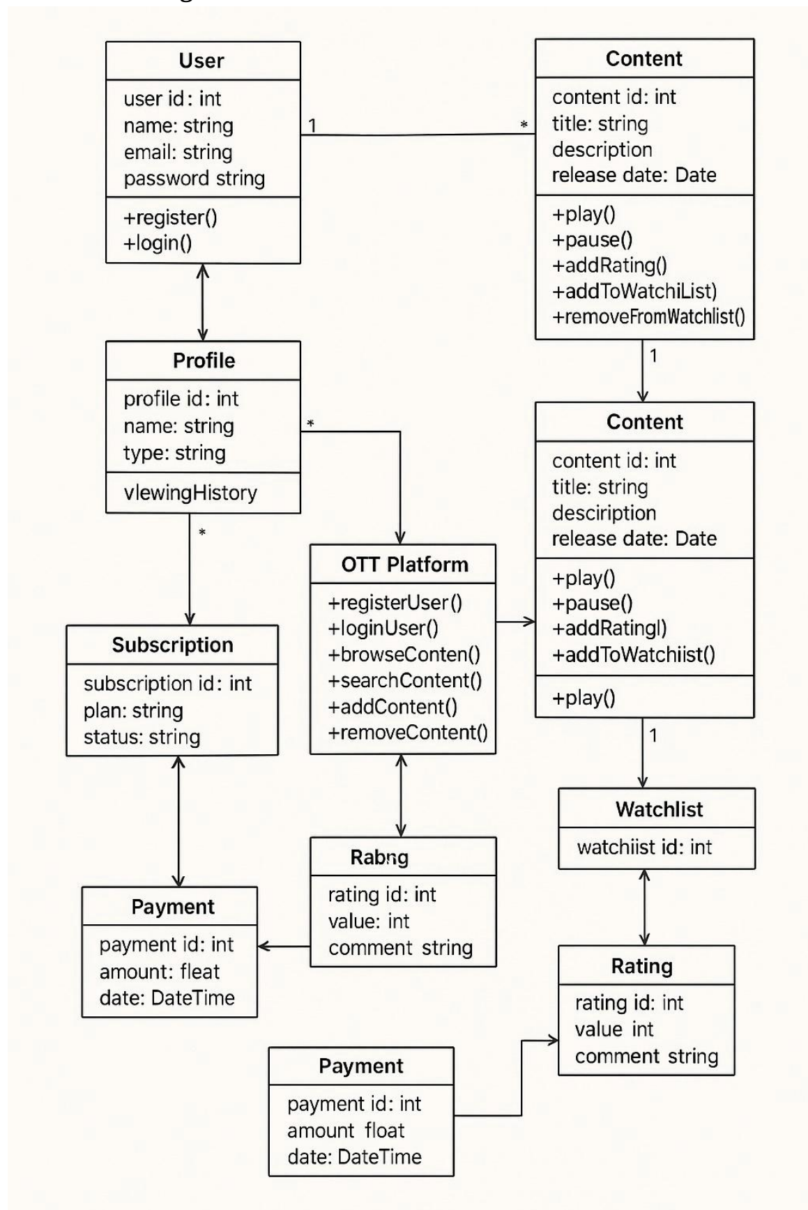
5.7 UML Class Diagram for OTT Platform
