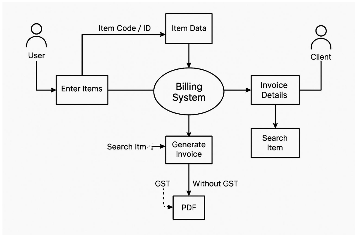
5.4 Level 1 Billing System DFD Diagram
